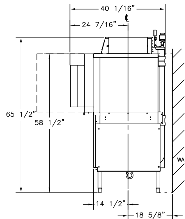
VIEW D-D
