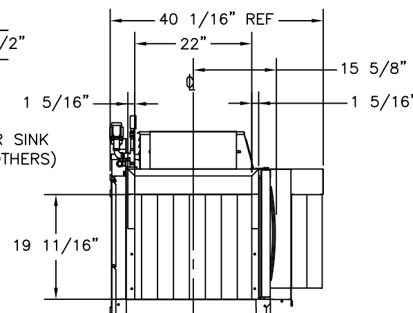
VIEW D-D
